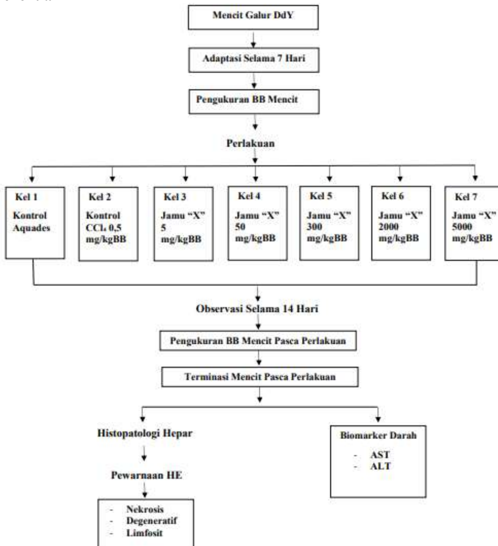
Gambar 1. Alur Penelitian
