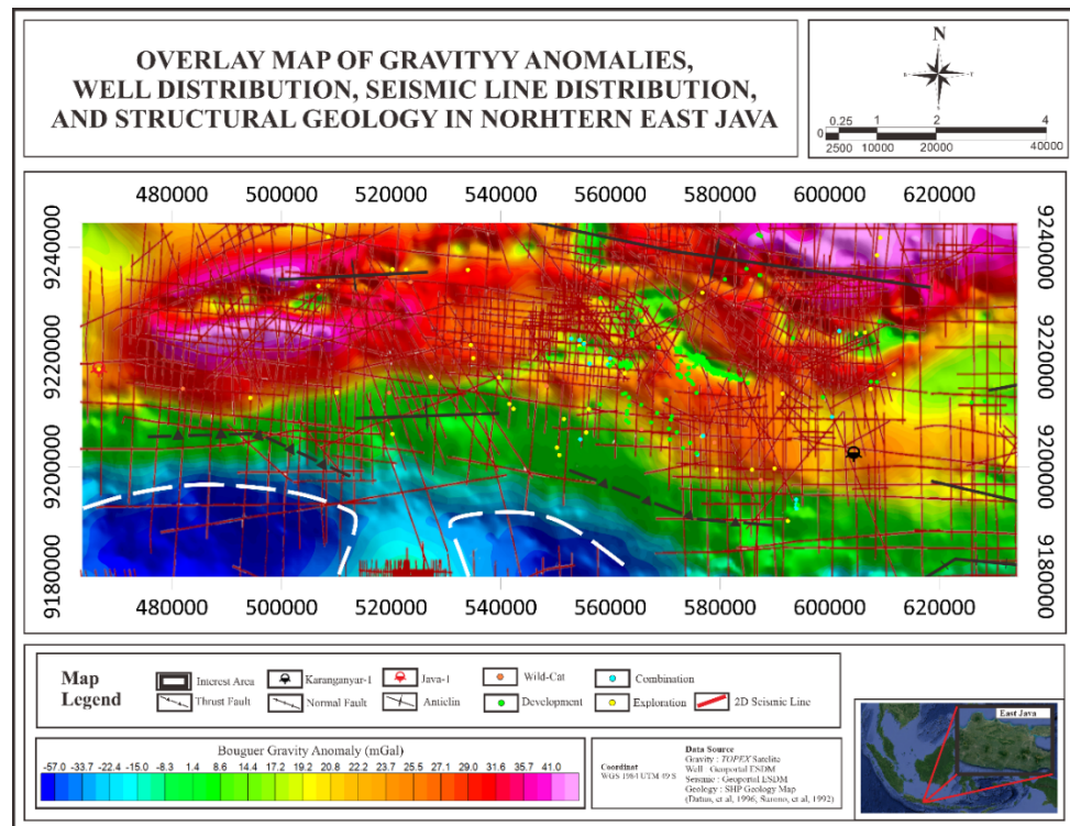
Figure 5. Overlay map of gravity anomalies, well distribution, line distribution, and structural geology in Northern East Jawa
